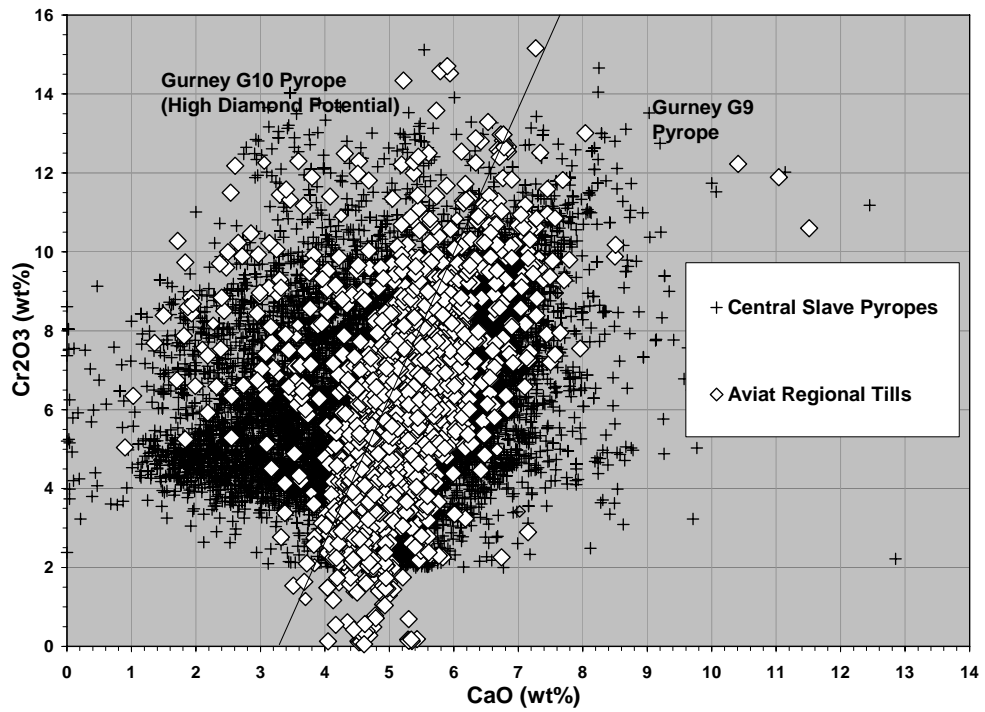
CaO vs Cr2O3 For Peridotitic Garnets From The Aviat Project
