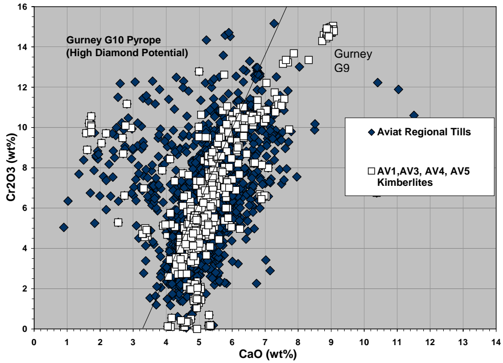
CaO vs Cr2O3 For Peridotitic Garnets From The Aviat Project
